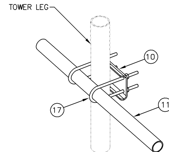
TIE BACK DETAIL AT TOWER LEG
