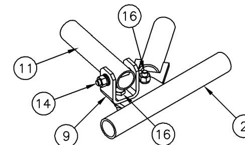
TIE BACK DETAIL AT ANTENNA MOUNTING FRAME
